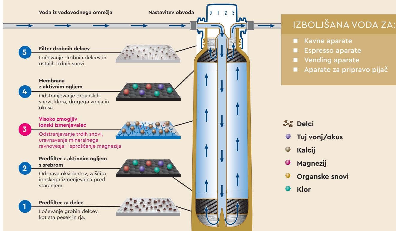
FILTRIRNA KARTUŠA BWT BESTMAX PREMIUM
